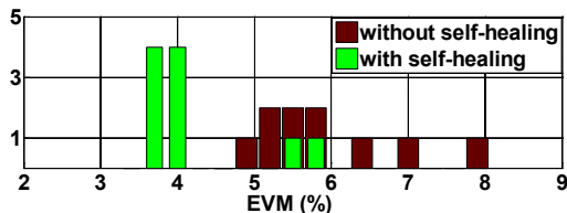
Fig. 7 EVM histogram for 10 chips at 12.5dBm output power and 100ksps 16QAM modulation before and after healing.
