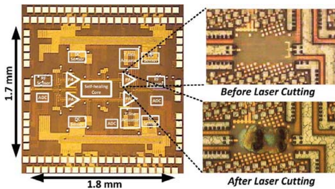
Fig. 35. Chip photograph showing functional blocks, and close-up of the output stage before and after laser cutting.
