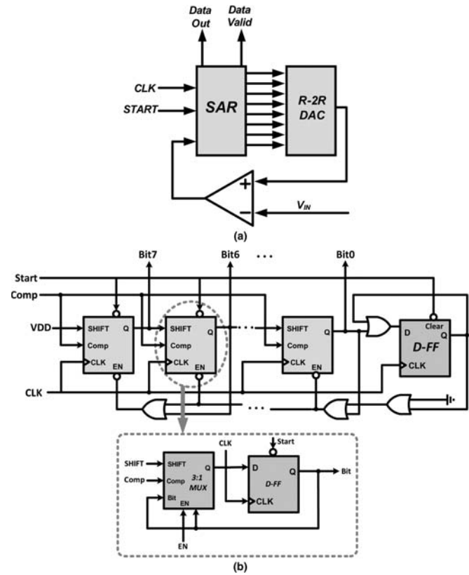
Fig. 23. (a) Block diagram of SAR ADC. (b) Synchronous SAR block.
