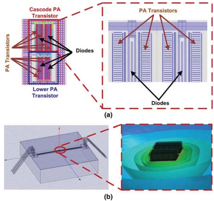
Fig. 17. (a) Layout of the PA transistor with the interspersed diodes in between and (b) the simulated thermal profile for 80-mW power dissipation in the process.
