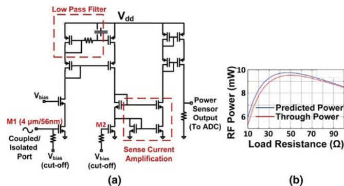
Fig. 12. (a) Power detector schematic showing rectification, low-pass filtering, and current amplification. (b) Simulated predicted and through power of the RF power sensor.
