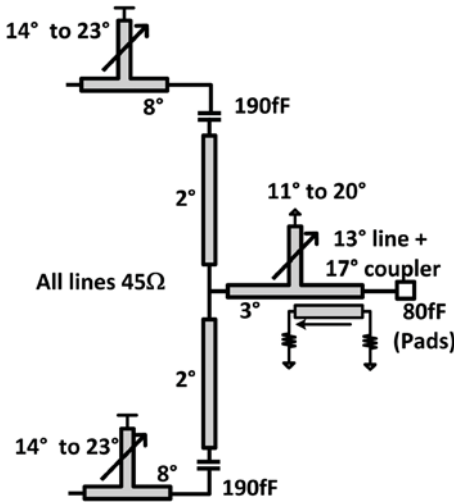
Fig. 4. Schematic of the output power-combining matching network.
